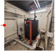
Rainwater Storage Tank
